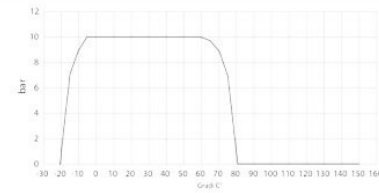
DIAGRAMMA PRESSIONE TEMPERATURA VIP FKM VIP FPM PRESSURE TEMPERATURE DIAGRAM
