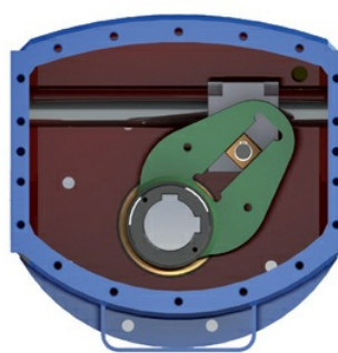
DESIGN SIMMETRICO SYMMETRICAL DESIGN
