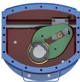
DESIGN ASIMMETRICO CANTED DESIGN
